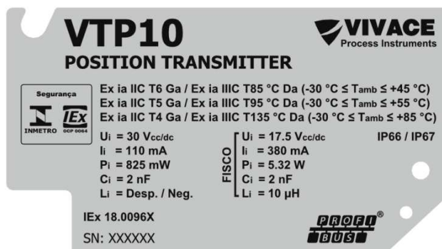
Figura 5.2 – Plaqueta Ex ia do VTP10-P.
